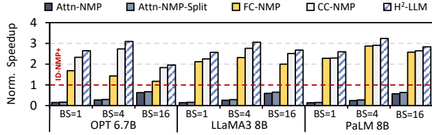
Figure 13: Dataflow Designs on H 2 -LLM v.s. ID-NMP+.
