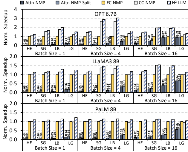
Figure 12: Comparison Against Existing Dataflow Designs.
